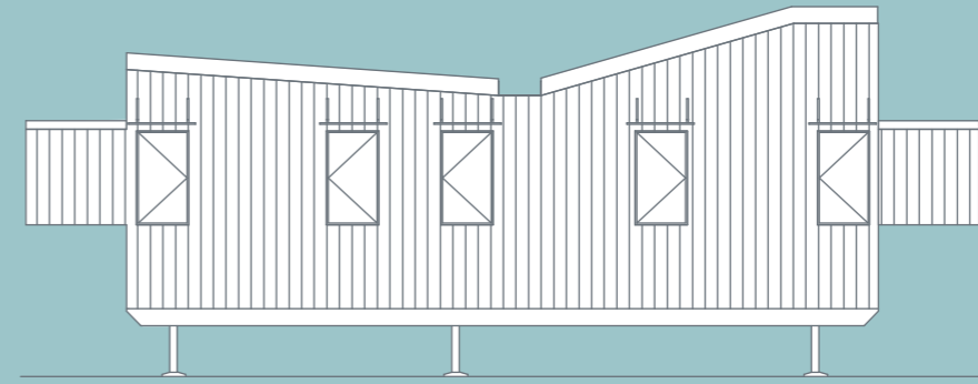
2 ELEVATION EXPANDER STUDIO
