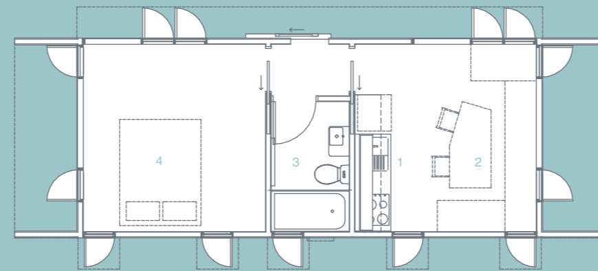
1 FLOOR PLAN EXPANDER STUDIO
