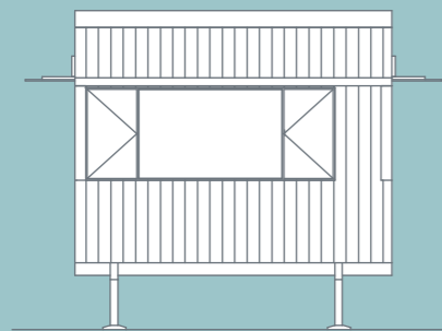
5 ELEVATION EXPANDER STUDIO
