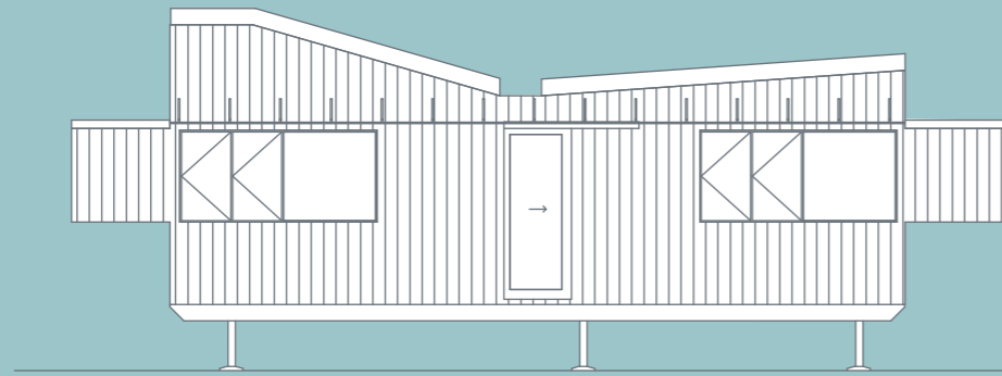
3 ELEVATION EXPANDER STUDIO
