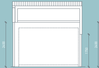
4 ELEVATION CARSHED
