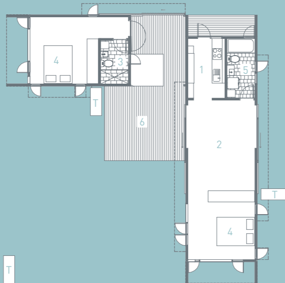
2 FLOOR PLAN 2 BED HOUSE
