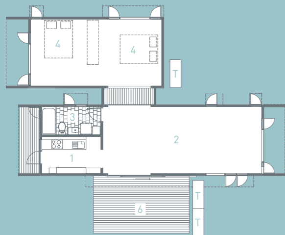
3 FLOOR PLAN 2 BED HOUSE
