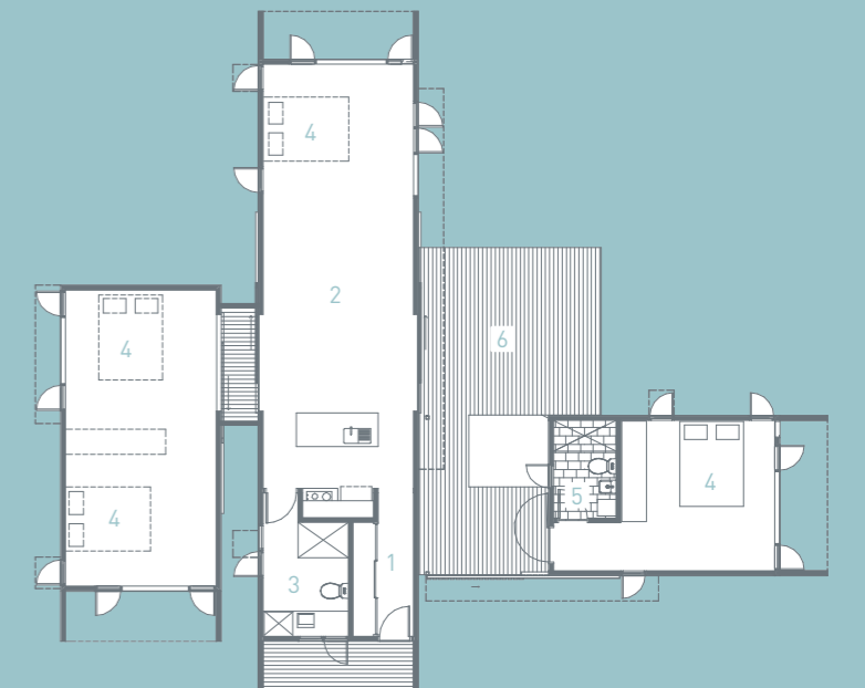
7 FLOOR PLAN 4 BED HOUSE
