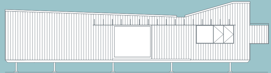
2 ELEVATION GALLEY
