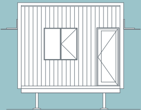
5 ELEVATION GALLEY
