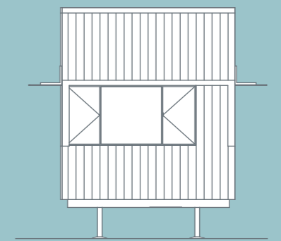
4 ELEVATION SLIM
