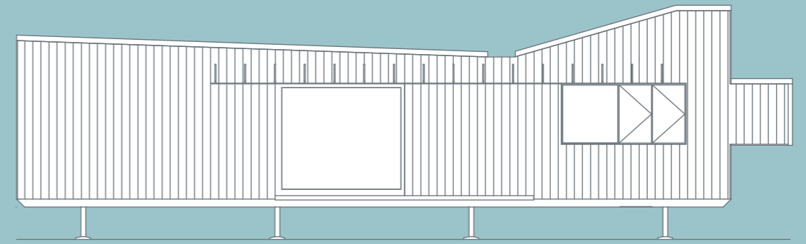
5 ELEVATION SLIM
